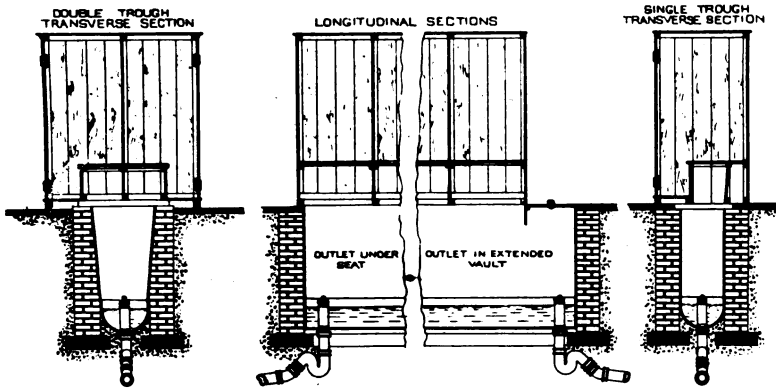
FIGURE 46 A SCHOOL-SINK
