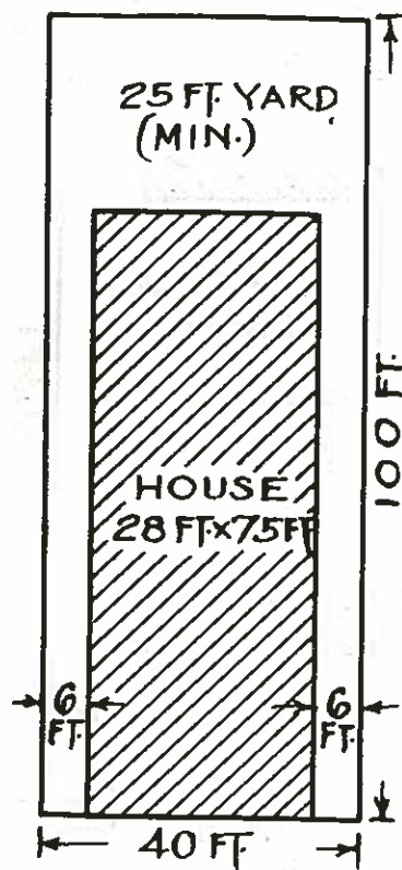
FIGURE 55 THREE-STORY AND ATTIC
