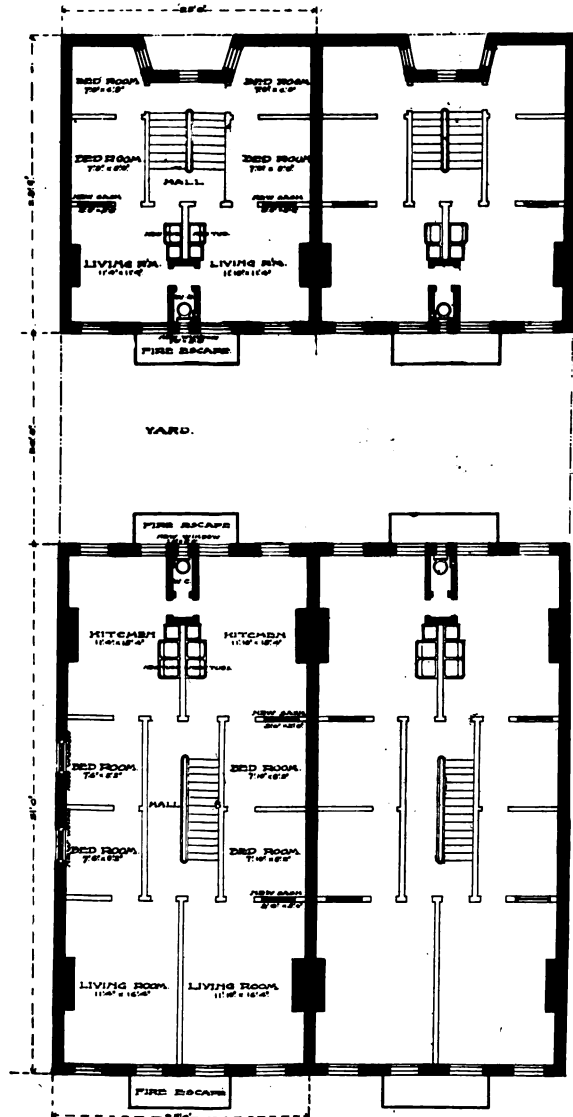
FIGURE 40 PUTTING WATER-CLOSETS INSIDE THE HOUSE BETWEEN TWO FLATS IN A FRONT AND REAR HOUSE
