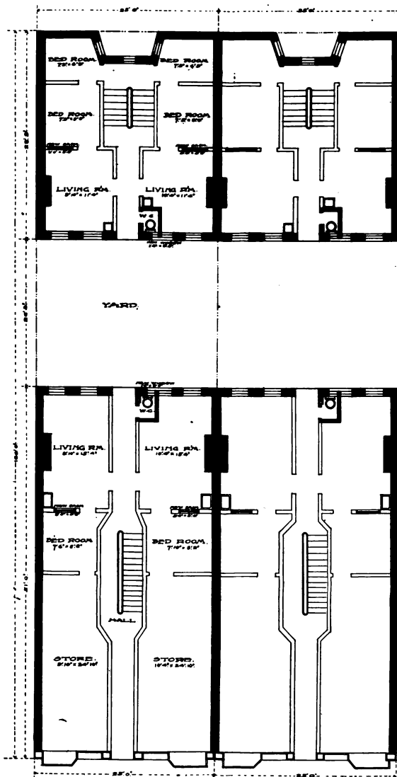
FIGURE 41 PUTTING WATER-CLOSETS INSIDE THE HOUSE OFF THE PUBLIC HALL PLAN OF ENTRANCE FLOOR
